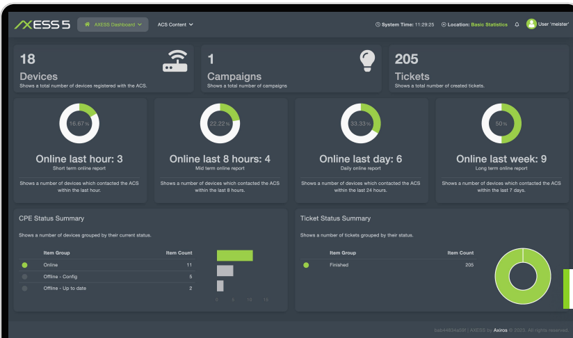
AXESS simple statistics
